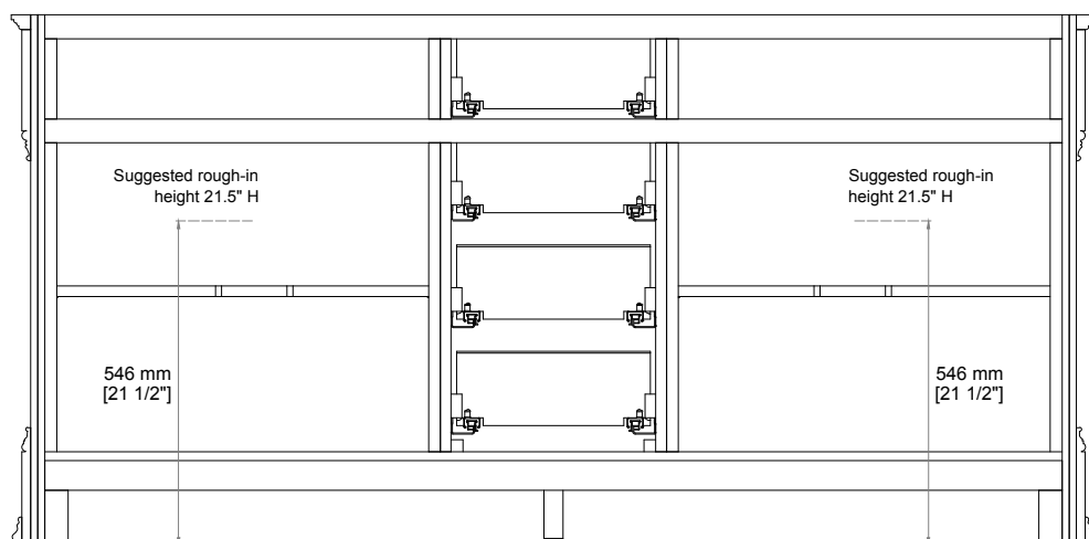
Back View
