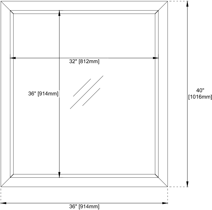
Front View
